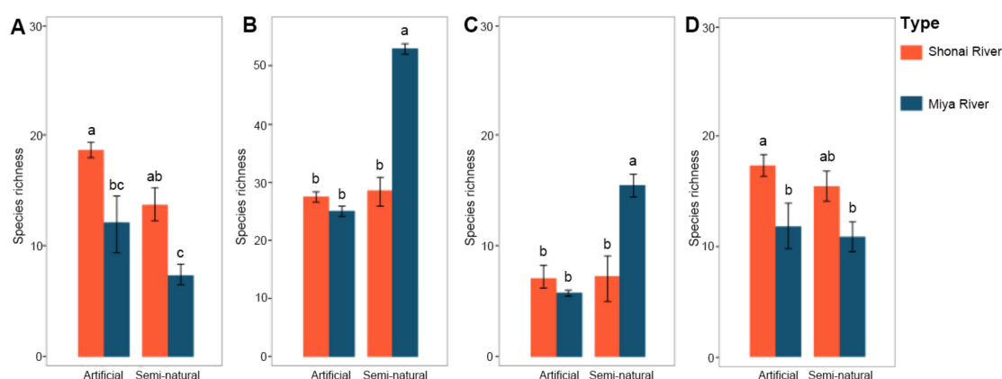
Figure 4. The number of plant species across habitat types and rivers in alien species richness (A), native species richness (B), riparian species richness (C), and ruderal species richness (D). Shown are means \pm standard error. Letters represent significant differences ( p \leq 0.05 , the p -values were corrected by the multiple-testing Holm's correction).
